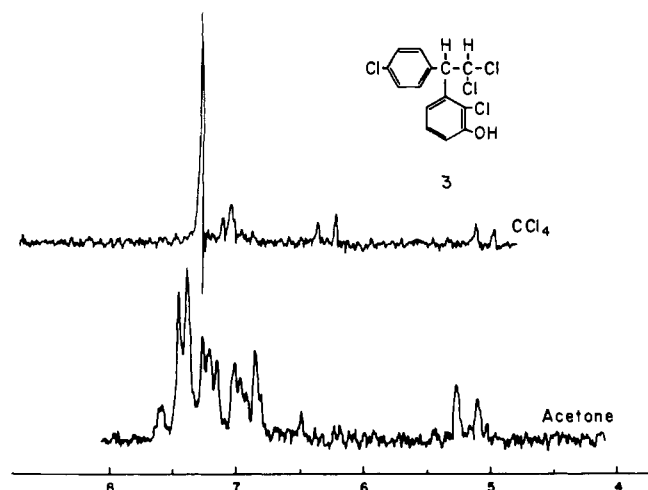
Figure 4. 60 MHz nmr spectra of metabolite 3 in carbon tetrachloride and acetone- d_6 .
